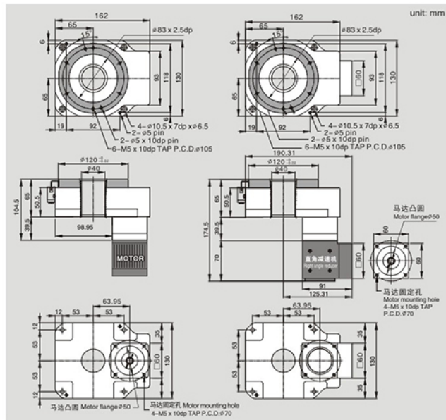
60 型步进马达定置 减速比=1:30 60 TYPE STEPPING MOTOT RATING Speed reduction ratio=1:30
