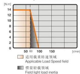
200-400W伺服马达定置 减速比=1:30 200-400W SERVO MOTOT RATING Speed reduction ratio=1:30
